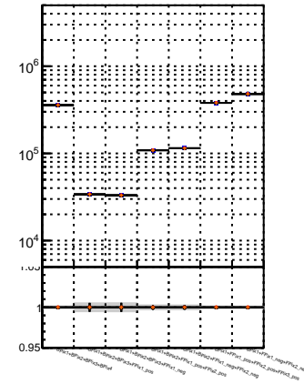
N of reco track vs. \chi^2 mxFit-13.0.0e4 Overlap-check-chi2-50 Overlap-check-chi2-1000
