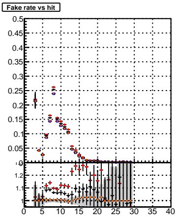
— mkFit_13.0.0p4 —+ overlap-check-chi2-60 —+ overlap-check-chi2-1100 —+ overlap-check-chi2-10000
