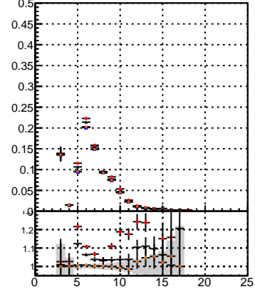
— mkFit_13.0.0p4 —+ overlap-check-chi2-60 —+ overlap-check-chi2-1100 —+ overlap-check-chi2-10000
