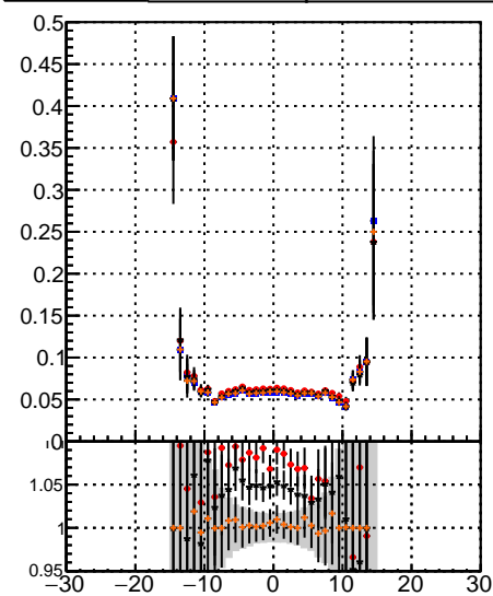
Fake rate vs dxy —●— mtFit-13.0.9p4 —●— overlap-check-ch12-60 —●— overlap-check-ch12-10000
