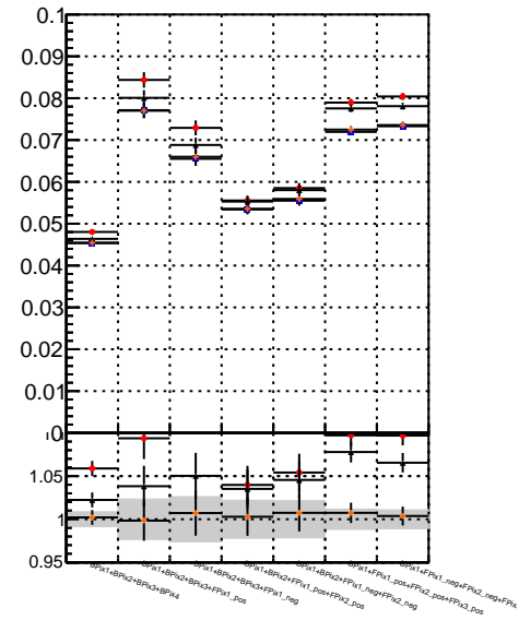
Fake rate vs. - m_k \text{Fit} = 13.0 \pm 0.4 - \text{overlap\_check\_chiz-60} - \text{overlap\_check\_chiz-10000}
