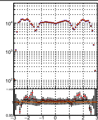
N of reco track vs \eta bkFit 13.0.0e4 overlap-check-chi2-60 overlap-check-chi2-1000
