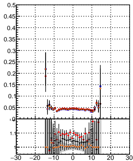
Fake rate vs dxy mtFit-13.0.0p4 overlap-check-ch12-60 overlap-check-ch12-10000
