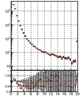
N of reco track vs. \chi^2 mxFit-13.0.0e4 overlaid-check-chi2-50 overlaid-check-chi2-1000
