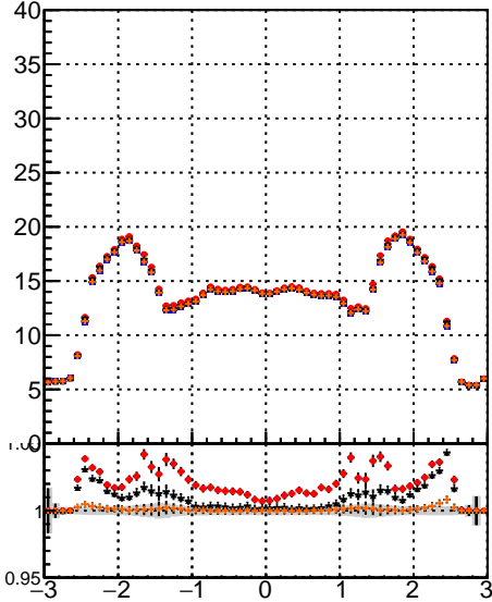
mean hit
