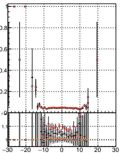
Fake rate vs d mtFit-13.0.0p4 overlap-check-ch12-60 overlap-check-ch12-10000
