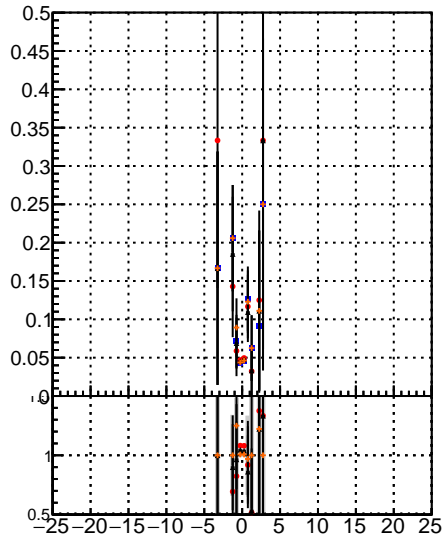
Fake rate vs d mtFit-13.0.0p4 overlap-check-ch12-60 overlap-check-ch12-10000
