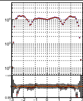
bkFit-13.0.0-4 overlap-check-chi2-60 overlap-check-chi2-1000
