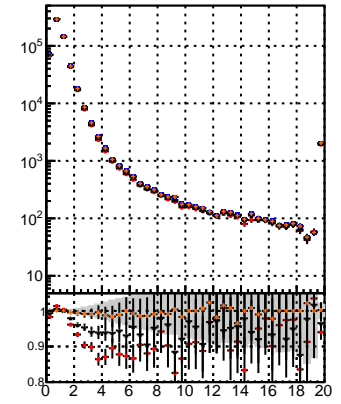
N of associated (recoSim) tracks vs normalized \chi^2
