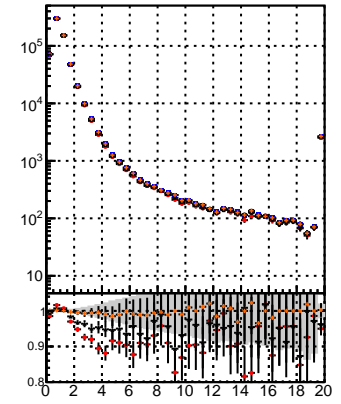
N of reco track vs. \chi^2 ● mkrFit-13.0.0e4 ● Overlap-check-chi2-50 ● Overlap-check-chi2-1000 ■ verBat
