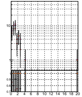
N of associated (recoSim) looper tracks vs normalized \chi^2
