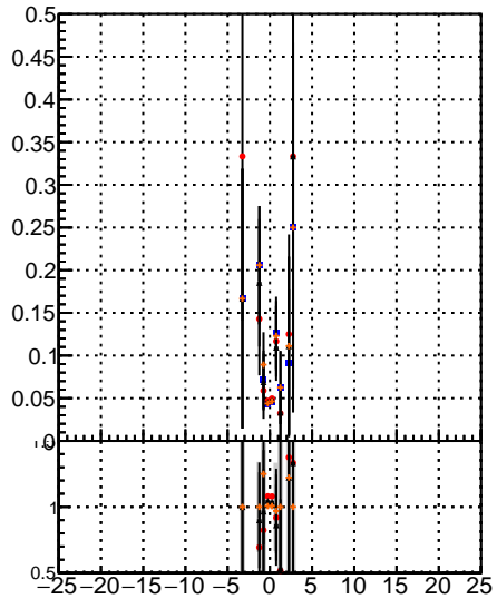
Fake rate vs dxy mFit-13.0.0p4 overlap-check-ch12-60 overlap-check-ch12-10000
