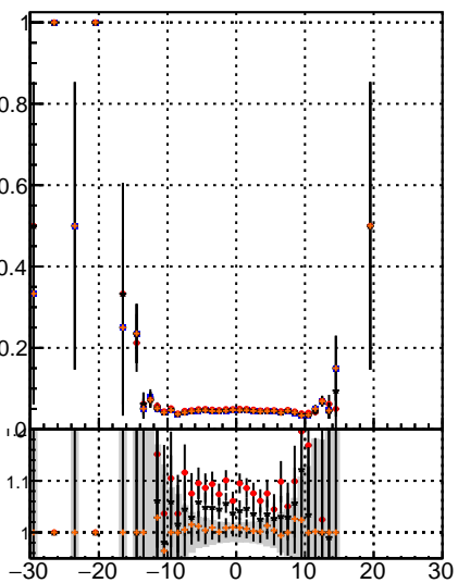
Fake rate vs dxy mFit-13.0.0p4 overlap-check-ch12-60 overlap-check-ch12-10000
