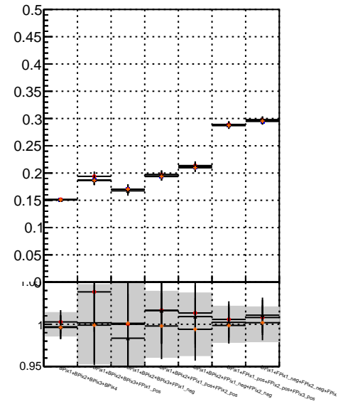
Fake rate vs. - m_k Fit - 13.0.9p4 - \chi^2 - 60 - \chi^2 - 10000
