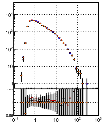
muFit-13.0.0-04 overlap-check-ch12-60 overlap-check-ch13-1000
