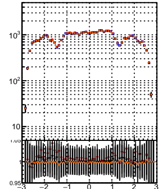
muFit-13.0.0-04 overlap-check-ch12-60 overlap-check-ch13-1000
