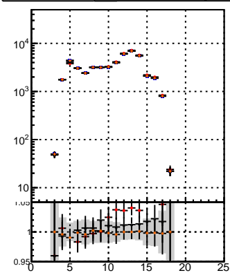
mkFit_13.0.0p4 overlap-check-chi2-60 overlap-check-chi2-1000 overlap-check-chi2-10000
