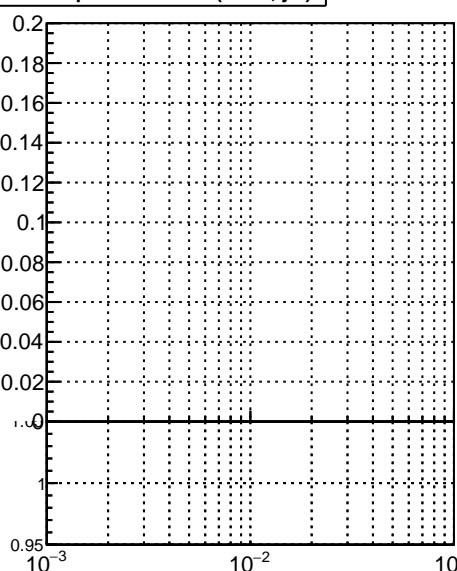
fake+duplicates vs \Delta R (track, jet)
