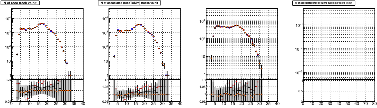
Legend for top row plots: mkFit_13.0.0p4 overlap-check-chi2-60 overlap-check-chi2-1000 overlap-check-chi2-10000
