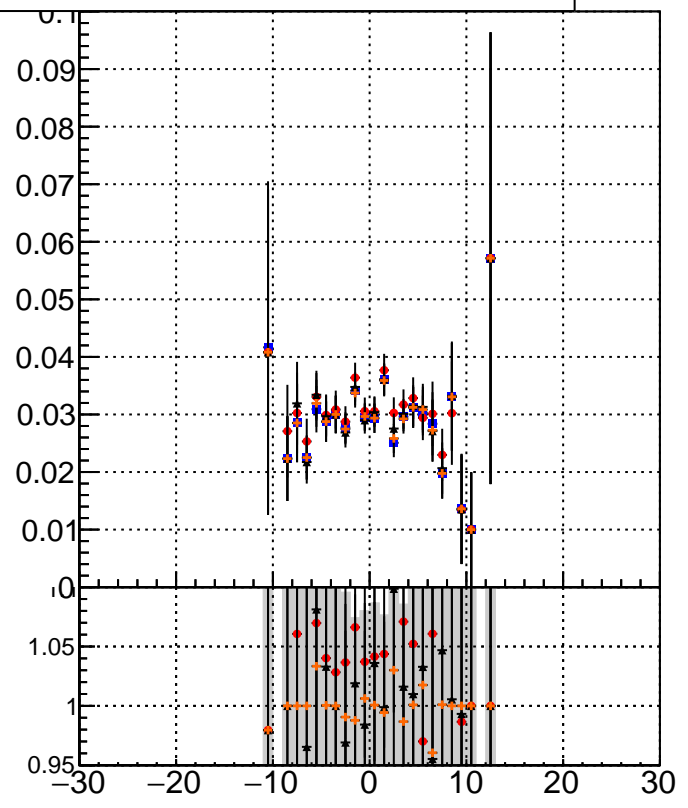
Legend for the plots: mkFit_13.0.0p4 overlap-check-chi2-60 overlap-check-chi2-1100 overlap-check-chi2-10000
