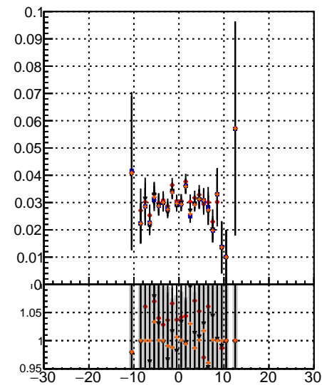
Fake rate vs d mlFit - 13.0.9e4 overlap-check-chiz-60 overlap-check-chiz-1000
