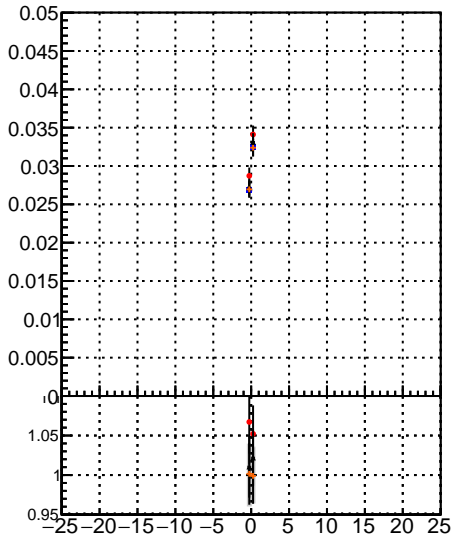
Fake rate vs d mlFit - 13.0.9e4 overlap-check-chiz-60 overlap-check-chiz-1000
