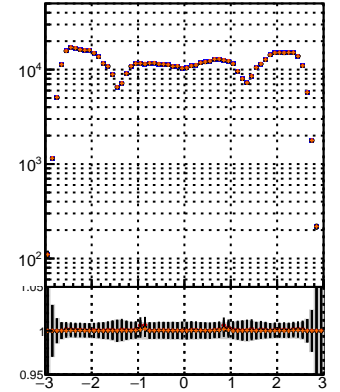
bkFit-13.0.0-4 overlap-check-chi2-60 overlap-check-chi2-1000 N of reco track vs \eta
