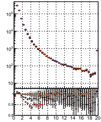
N of reco track vs. \chi^2 mkFit-13.0.0e4 overlap-check-chi2-50 overlap-check-chi2-1000
