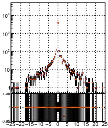
N of sim — mkFit_13.0.0p4 — overlap-check-chi2-60 — overlap-check-chi2-1100 — overlap-check-chi2-10000
