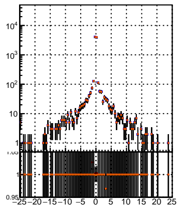
— mkFit_13.0.0p4 — overlap-check-chi2-60 — overlap-check-chi2-1100 — overlap-check-chi2-10000 N of sim
