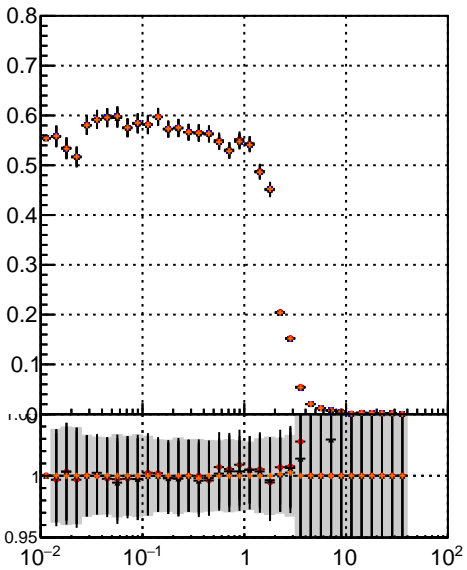
Efficiency —●— mkFit_13.0.0p4 —◆— overlap-check-chi2-60 —▲— overlap-check-chi2-1100 —◆— overlap-check-chi2-10000
