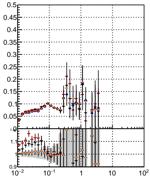
Efficiency —●— mkFit_13.0.0p4 —◆— overlap-check-chi2-60 —▲— overlap-check-chi2-1100 —◆— overlap-check-chi2-10000
