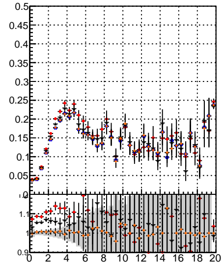
Fake rate vs. - \chi^2 fit: 13.0 994 - overlap-check-chi2-60 - overlap-check-chi2-10000
