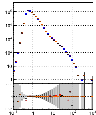
bkFit-13.0.0-4 overlap-check-chi2-60 overlap-check-chi2-1000
