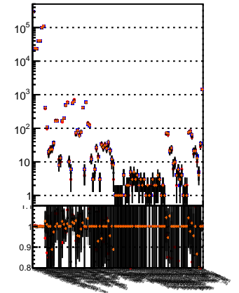
N of reco track vs. \chi^2 ● mkrFit-13.0.0e4 ● Overlap-check-chi2-50 ● Overlap-check-chi2-1000
